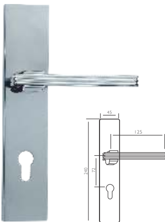
CP Mirror L17-593PP
